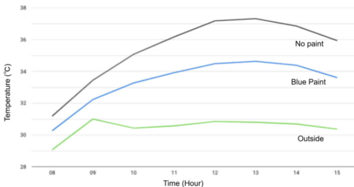
Figure 30: Minute by minute temperature recordings averaged across the four days and averaged hourly, from 19th December 2021 - 22nd December 2022 for the Blue Paint Intervention Classroom, Control Classroom and Outside under a tree.
