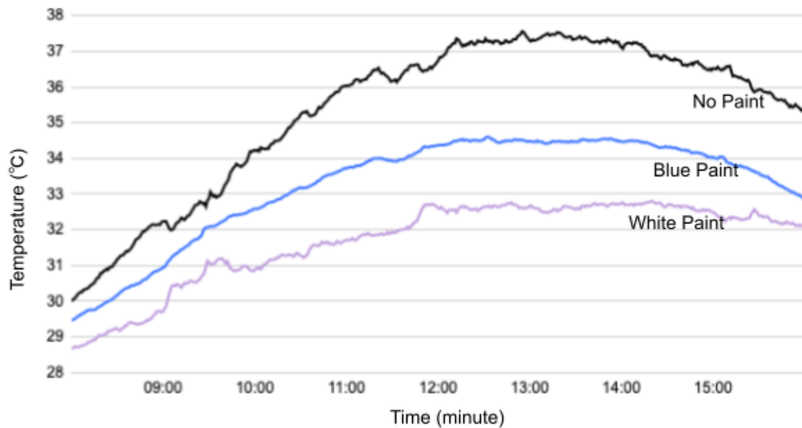
Figure 32: Minute by minute temperature recordings modelled and averaged across the 8 days for the White Paint Intervention Classroom, Blue Paint Intervention and Control Classroom.
