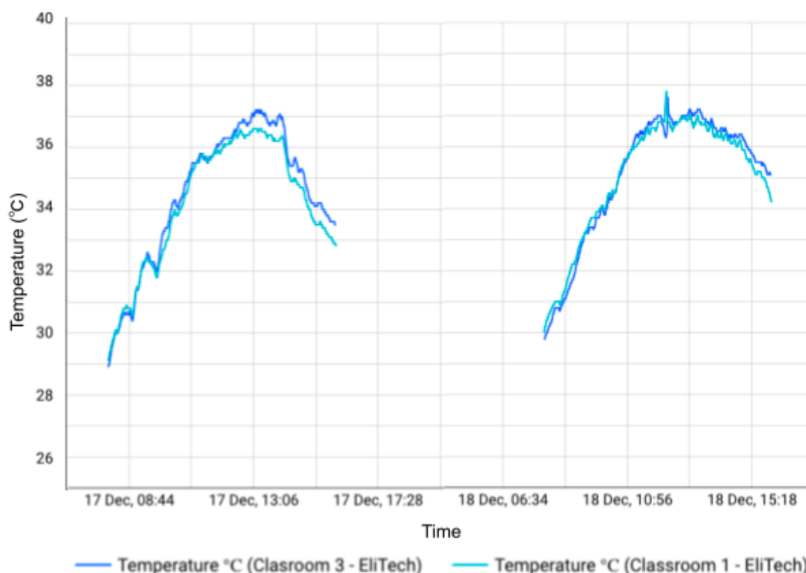
Figure 27: Graph showing the calibration temperatures recorded over the course of two days, during school hours, in Classroom C1 and Classroom C3.
