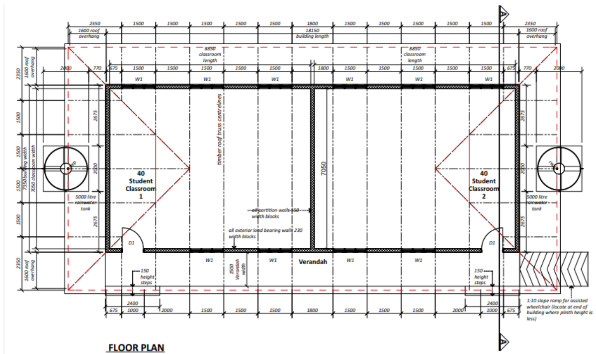
Figure 6: Floor plan of a standard two classroom block construction.
