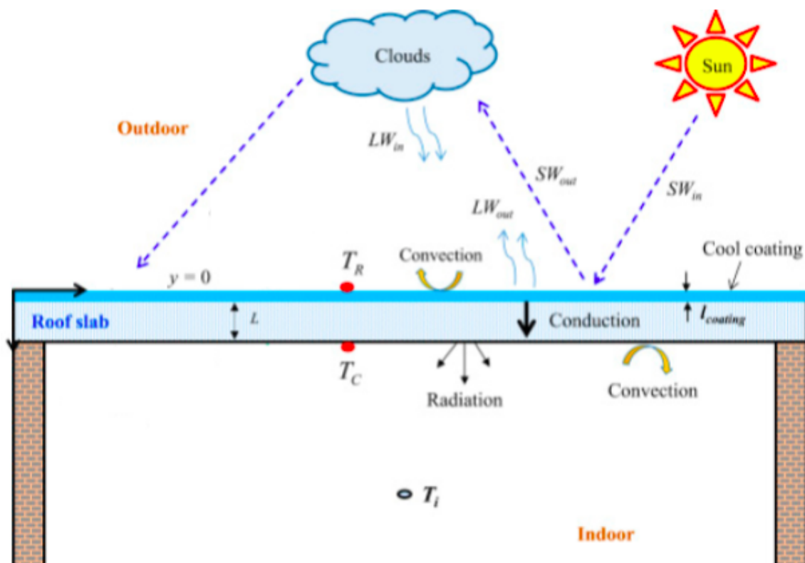
Figure 10: Showing the movement of heat through a roof. The roof shown here is a flat roof, but the same heat flow processes apply to a sloped roof on a classroom block. The Incident (I) radiation on the roof is given by assessing the short wave radiation (SW) radiation directly from the sun and the longwave radiation (LW), reflected from clouds and the atmosphere. Equation (2) governs the radiation absorbed by the roof. Equation (3) gives the relationship of the heat transfer across the roof, accounting for emittance and reflectivity.
