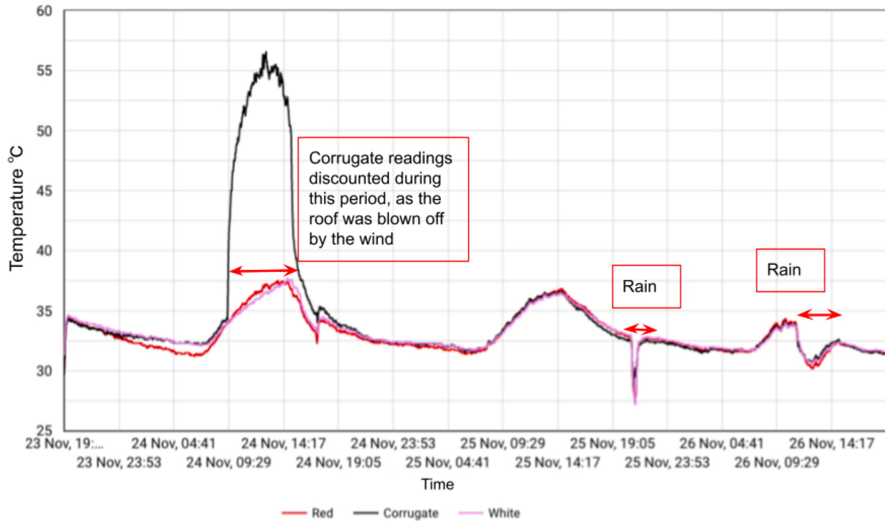
Figure 19: Showing the temperature recorded in each of the model classrooms over the course of the three days.
