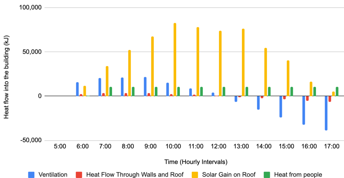
Figure 9: Heat flow into the building at hourly intervals - extracted from a proposed model for a classroom block in Malawi.
