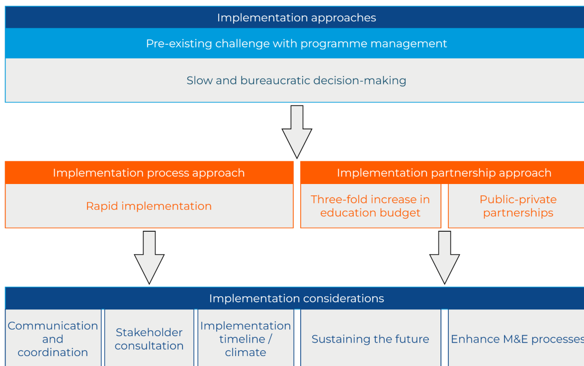
Figure 9. Programme management
